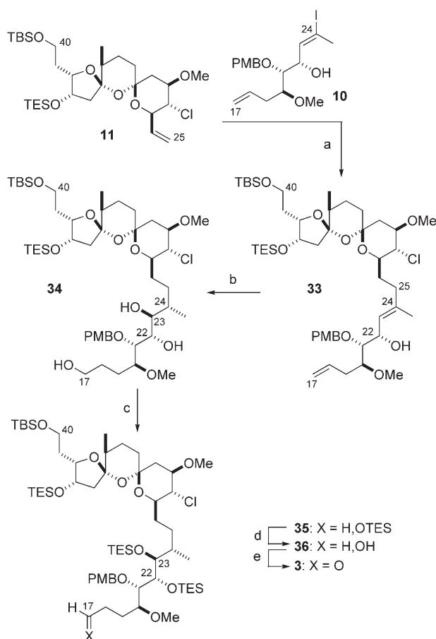
Scheme 7. Suzuki coupling reaction of alkene 11 and iodide 10 : formation of the fully functionalized C17–C40 aldehyde 3 . a) 9-BBN, THF; \text{H}_2\text{O} ; 10 , [\text{PdCl}_2(\text{dppf})] , \text{Ph}_3\text{As} , \text{Cs}_2\text{CO}_3 , THF/DMF (1:1), 83%; b) \text{BH}_3\cdot\text{SMe}_2 , THF; MeOH, 30% \text{H}_2\text{O}_2 , 1 M NaOH, 0^\circ\text{C} to RT; c) TESOTf, 2,6-lutidine, \text{CH}_2\text{Cl}_2 , -78^\circ\text{C} , 67% (over 2 steps, d.r. 75:25); d) PPTS, \text{CH}_2\text{Cl}_2/\text{MeOH} (12:1), 0^\circ\text{C} , 98%; e) DMP, \text{NaHCO}_3 , \text{CH}_2\text{Cl}_2 , 80%. 9-BBN = 9-borabicyclo[3.3.1]nonane, DMF = N,N -dimethylformamide, dppf = 1,1'-bis(diphenylphosphanyl)ferrocene.
