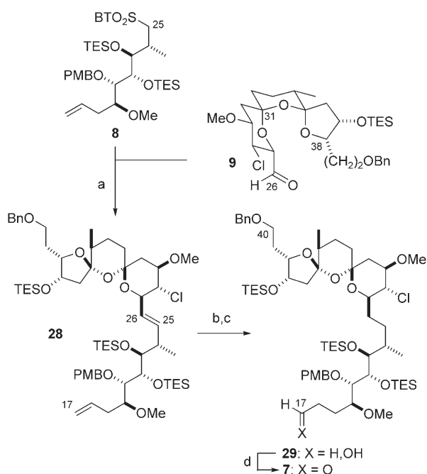
Scheme 5. Modified Julia olefination to form the C17–C40 subunit 7 . a) 8 , LHMDS, THF, -78^\circ\text{C} ; 9 , -78^\circ\text{C} to RT, 32%; b) \text{BH}_3\cdot\text{SMe}_2 , THF, 0^\circ\text{C} ; 30% \text{H}_2\text{O}_2 , pH 7 buffer; c) (\text{NCO}_2\text{K})_2 , AcOH, Py, MeOH, 81% (over 2 steps); d) DMP, \text{NaHCO}_3 , \text{CH}_2\text{Cl}_2 , 84%. LHMDS = lithium hexamethyldisilazide.
