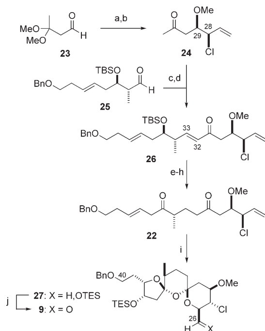
Scheme 4. Improved route to form the C26–C40 aldehyde 9 . a) \text{CH}_2=\text{CHCH}_2\text{Cl} , \text{cHex}_2\text{NLi} , (–)- \text{lpcBOMe} , THF, \text{Et}_2\text{O} , -95^{\circ}\text{C} ; \text{BF}_3\cdot\text{Et}_2\text{O} ; 23 , -95^{\circ}\text{C} to -78^{\circ}\text{C} ; 30% \text{H}_2\text{O}_2 , pH 7 buffer; b) \text{Me}_3\text{OBF}_4 , proton sponge, \text{CH}_2\text{Cl}_2 , 0^{\circ}\text{C} , 39% (over 2 steps); c) \text{cHex}_2\text{BCL} , \text{Me}_2\text{NEt} , \text{Et}_2\text{O} , 0^{\circ}\text{C} ; 25 , -78^{\circ}\text{C} , 88%; d) \text{MsCl} , \text{Et}_3\text{N} , 0^{\circ}\text{C} to RT, 83%; e) [(\text{Ph}_3\text{P})\text{CuH}]_d , \text{PhSiH}_3 , toluene, 90%; f) DIBALH, \text{CH}_2\text{Cl}_2 , -78^{\circ}\text{C} ; g) 1 N HCl, MeCN, RT; h) DMSO, (\text{COCl})_2 , \text{Et}_3\text{N} , \text{CH}_2\text{Cl}_2 , -78^{\circ}\text{C} to 0^{\circ}\text{C} , 75% (over 3 steps); i) see Ref. [4d], 65%; j) PPTS, \text{CH}_2\text{Cl}_2/\text{MeOH} (6:1), 0^{\circ}\text{C} ; DMP, \text{NaHCO}_3 , \text{CH}_2\text{Cl}_2 , 78%. cHex = cyclohexyl, DIBALH = diisobutylaluminum hydride, DMSO = dimethyl sulfoxide, lpc = isopinocampheyl, Ms = methanesulfonyl, PPTS = pyridinium para -toluenesulfonate.
