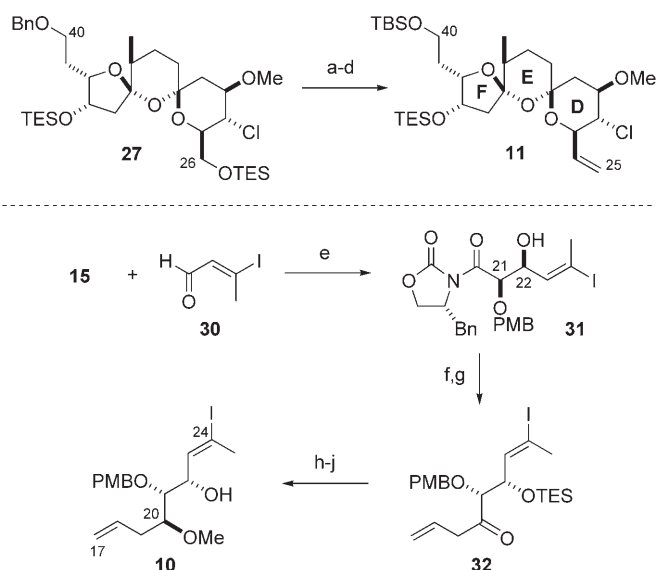
Scheme 6. Preparation of the C25–C40 alkene 11 and the C17–C24 vinyl iodide 10 . a) \text{H}_2 , Raney-Ni, EtOH; TBSCl, imidazole, \text{CH}_2\text{Cl}_2 , 86%; b) PPTS, \text{CH}_2\text{Cl}_2/\text{MeOH} (7:1), 0^\circ\text{C} ; c) DMP, \text{NaHCO}_3 , \text{CH}_2\text{Cl}_2 ; d) \text{Ph}_3\text{P}=\text{CH}_2 , THF, -78^\circ\text{C} to RT, 53% (over 3 steps); e) n\text{Bu}_4\text{BOTf} , \text{Et}_3\text{N} , toluene, -50^\circ\text{C} ; 30 , -50^\circ\text{C} to -30^\circ\text{C} , 79% (d.r. 95:5); f) \text{AlMe}_3 , \text{MeNH}(\text{OMe})\cdot\text{HCl} , THF, -20^\circ\text{C} to RT; TESOTf, 2,6-lutidine, \text{CH}_2\text{Cl}_2 , -78^\circ\text{C} , 86%; g) \text{CH}_2=\text{CHCH}_2\text{MgBr} , THF, -78^\circ\text{C} to 0^\circ\text{C} , 93%; h) Zn- (\text{BH}_4)_2 , \text{Et}_2\text{O} , -50^\circ\text{C} , 90% (d.r. > 95:5); i) \text{Me}_3\text{OBF}_4 , proton sponge, \text{CH}_2\text{Cl}_2 , 93%; j) PPTS, MeOH, 99%.
